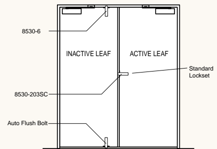
Double locking doors
