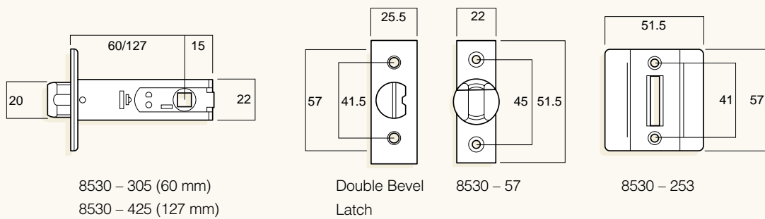
Double action push and pull doors
