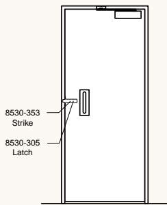
Single push and pull door
